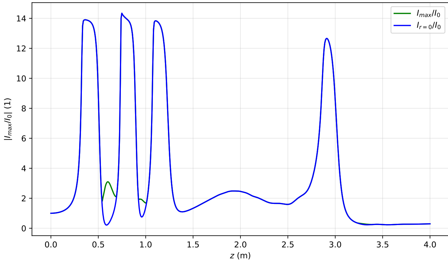
I_{max}(x = 0, y = 0, z)/I_0 , \text{Pin}=8.0\text{Pcr} , artificial time
